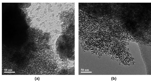
Fig. 3 TEM images of silica I (a) and IV (b).
