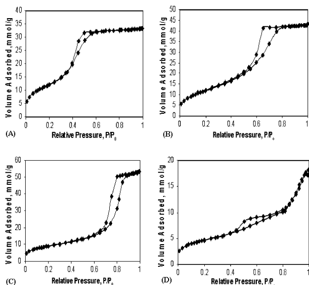
Fig. 4 Nitrogen adsorption-desorption isotherms recorded at 77 K for silicas I (A), II (B), III (C), and IV (D).
