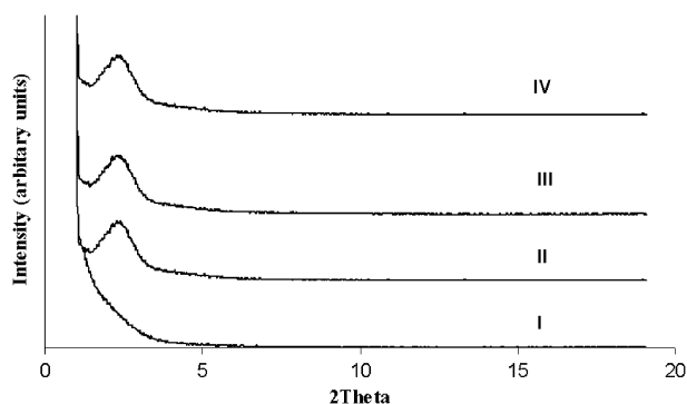
Fig. 2 X-Ray diffraction patterns of silicas I–IV .
